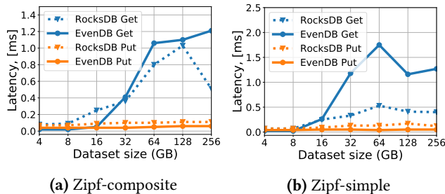
Figure 8. EvenDB vs RocksDB 95% latency (ms), under a mixed get-put workload A.
