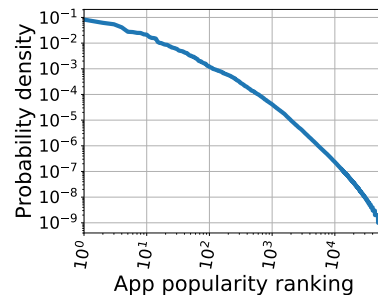
Figure 1. Distribution of mobile app events by app id (log scale) in a production analytics feed (2B events).
