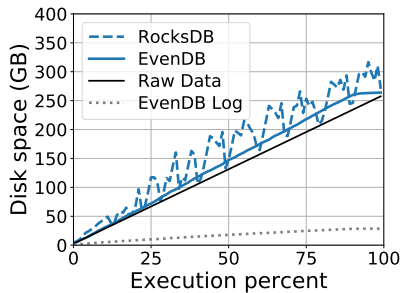
Figure 4. Space consumption during ingestion, 256GB.
